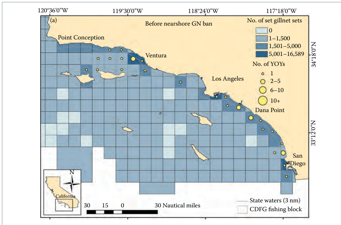
Figure 14.8 Spatial Distribution of set-gillnet effort and associated YOY White Shark Captures in Southern California before 1981-1993, a) and after (1994-2008, b) the nearshore-gillnet ban. The numbers represent sample sizes for fishing blocks with greater than 10 sharks. GN, gillnet.
